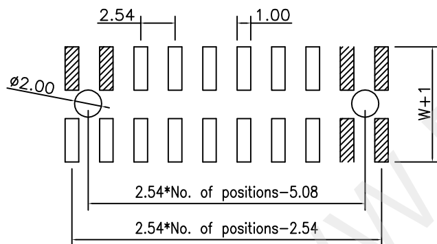
PCB LAYOUT
